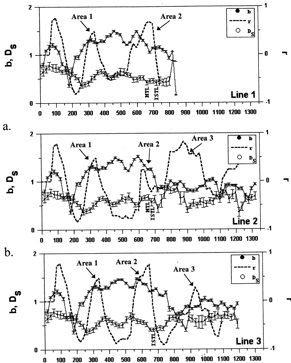
Figure 7. Variations in b and D_s along lines 1-3. MTL, Median Tectonic Line. ISTL, Itoigawa Shizuoka Tectonic Line. The dashed line shows variations in the local correlation between b and D_s . (a) Line 1 ending in central Japan. (b) Line 2 extending along the entire length of Honshu. (c) Line 3 extending along the entire length of Honshu. Area 1 through 3 are labeled.
