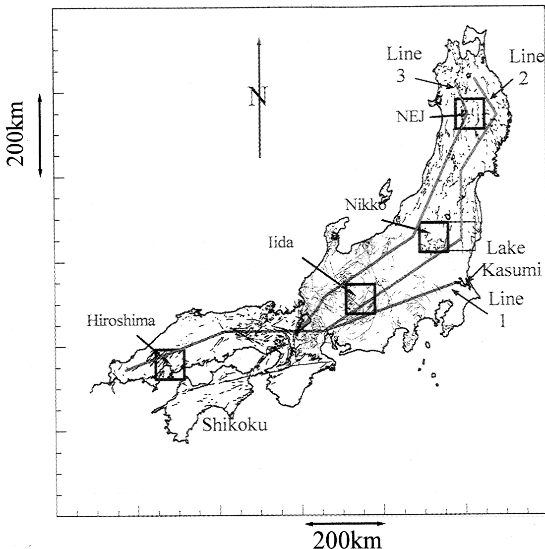
Figure 2. Active fault map of Honshu and Shikoku. The 70km x 70 km Hiroshima and Iida analysis areas are located along with analysis lines 1 through 3. Reference distances are marked on the analysis lines.
