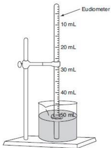
Eudiometer Tube or Gas Collecting Tube
