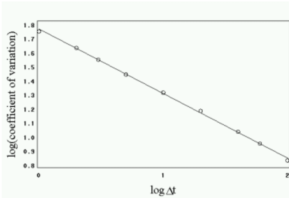
Figure 2. Power law for the coefficients of variation of slope -0.4588 over two orders of magnitude ( 1 \leq \Delta t \leq 100 ); a scaling index of 2.18 is implied.
