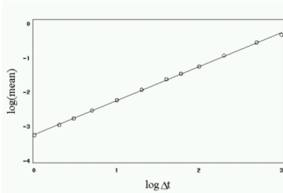
Figure 1. As the time lags are increased, a non-Gaussian power law emerges for the means within the time window of 1 \leq \Delta t \leq 1000 . In a log-log plot of mean against \Delta t a straight line of slope 0.990741 is reckoned. Given that a Lévy functional form seems to describe well the modal region of the distributions of the \Delta t considered, a scaling index of -1.0093 is implied.
