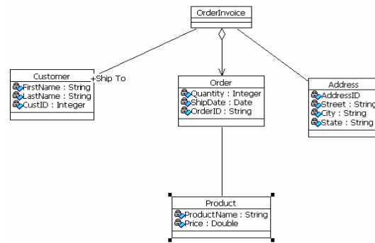
Fig 6 : Class model representing our sample XML Schema
