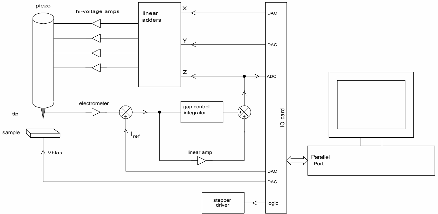
Fig. 2. System block diagram
