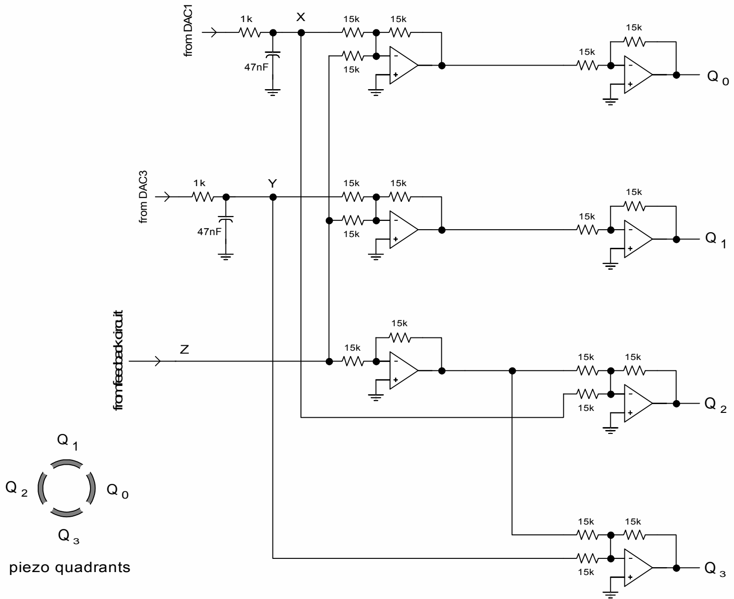
Fig. 11. Linear adders and scanning integrators.
