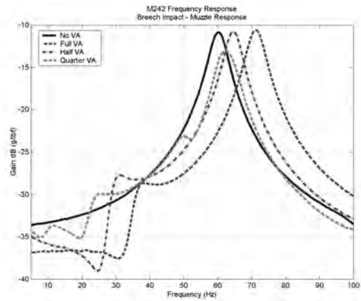
Figure 16. Frequency Response Comparison 0 to 100 Hz
