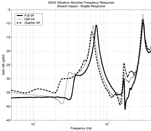
Figure 14. Vibration Absorber – Frequency Response
