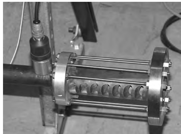
Figure 13. Installed Vibration Absorber
