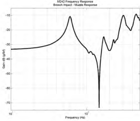
Figure 6. Plain Barrel – Frequency Response
