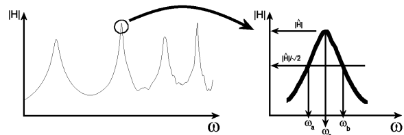
Figure 8. Peak Amplitude Method 5
