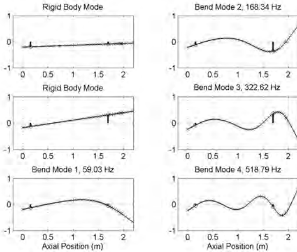
Figure 4. Damped Mode Shapes and Natural Frequencies
