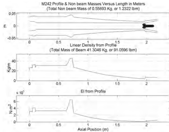
Figure 10. Barrel Geometry with Eight-Rod Vibration Absorber
