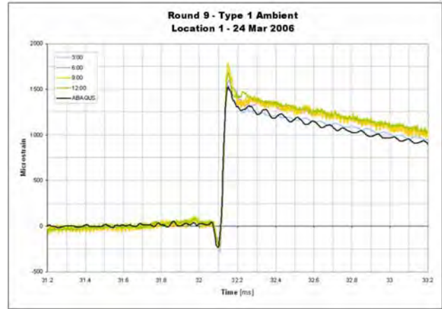
Figure 5–Experimental & Theoretical Strain vs. Time
