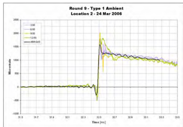
Figure 6–Experimental & Theoretical Strain vs. Time
