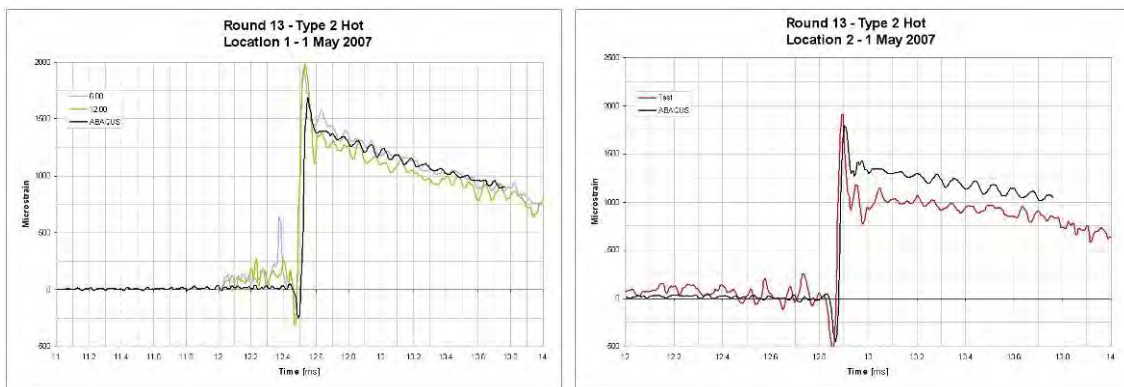
Figure 8–ATD-6 Location 1 (left) and Location 2 (right), Type 2, Strain vs. Time
