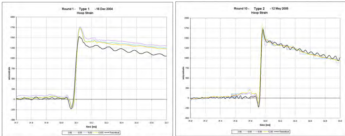
Figure 6–ATD-3 Location 1, Type 1 (left) and Type 2 (right), Strain vs. Time
