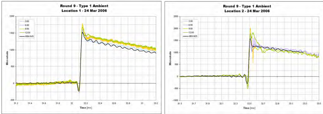
Figure 7–ATD-5 Location 1 (left) and Location 2 (right), Type 1, Strain vs. Time
