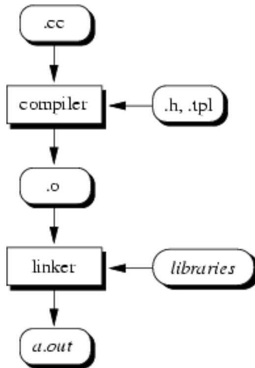
Figure 9.1: Compilation steps.
