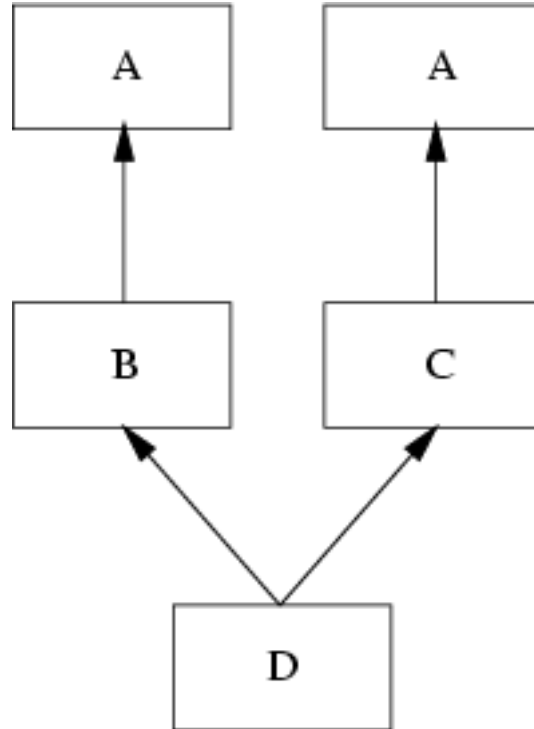
Figure 5.9: Illustration of the second multiple inheritance semantics.
