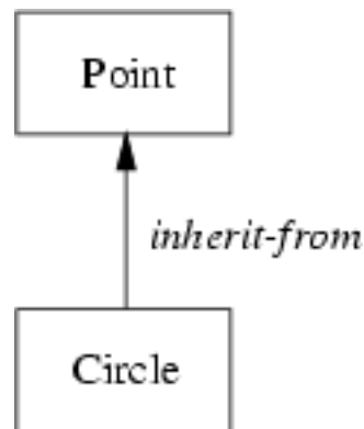
Figure 5.5: A simple inheritance graph.
