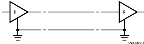
FIGURE 6. Typical TIA/EIA-694 Application
