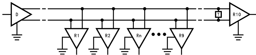
FIGURE 8. Typical TIA/EIA-422-B Multidrop Application
